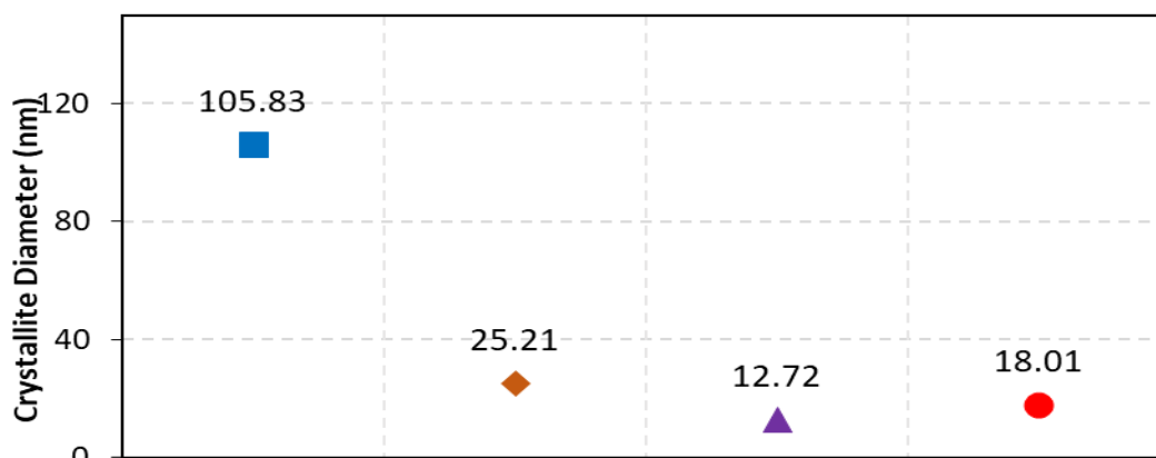
Figure 6 Crystallite diameter calculated by Williamson-Hall equation at FWHM values of (111) peaks detected by XRD.
