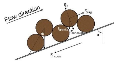
Figure 4 Forces acting on the particle at an active erosion site of a cuttings bed (adopted from Skalle, 2011 [43])
