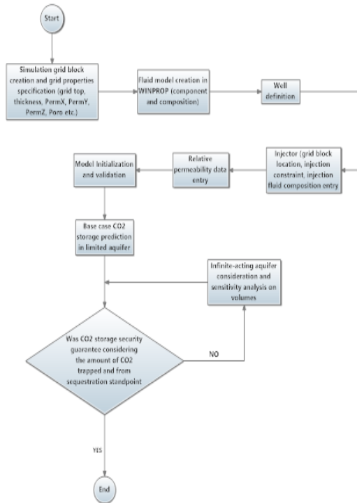
Figure 1 Simulation workflow
